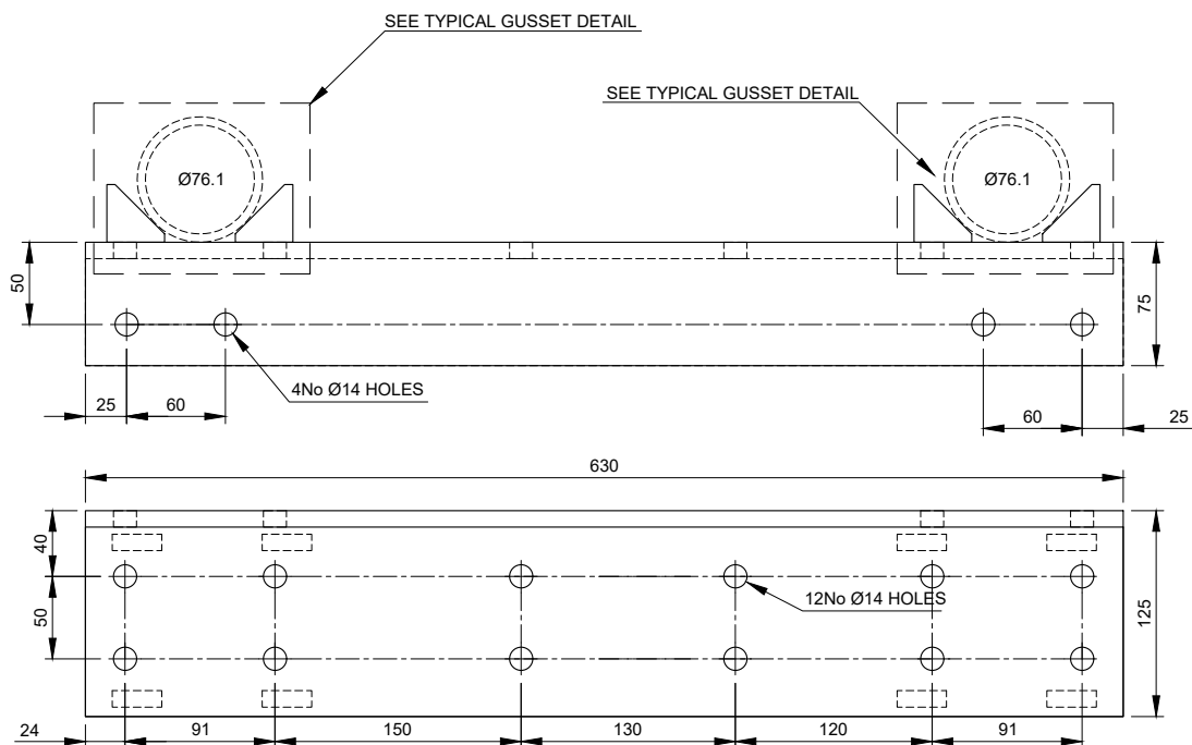
TPA-M - UA125x75x10 Scale 1:5
