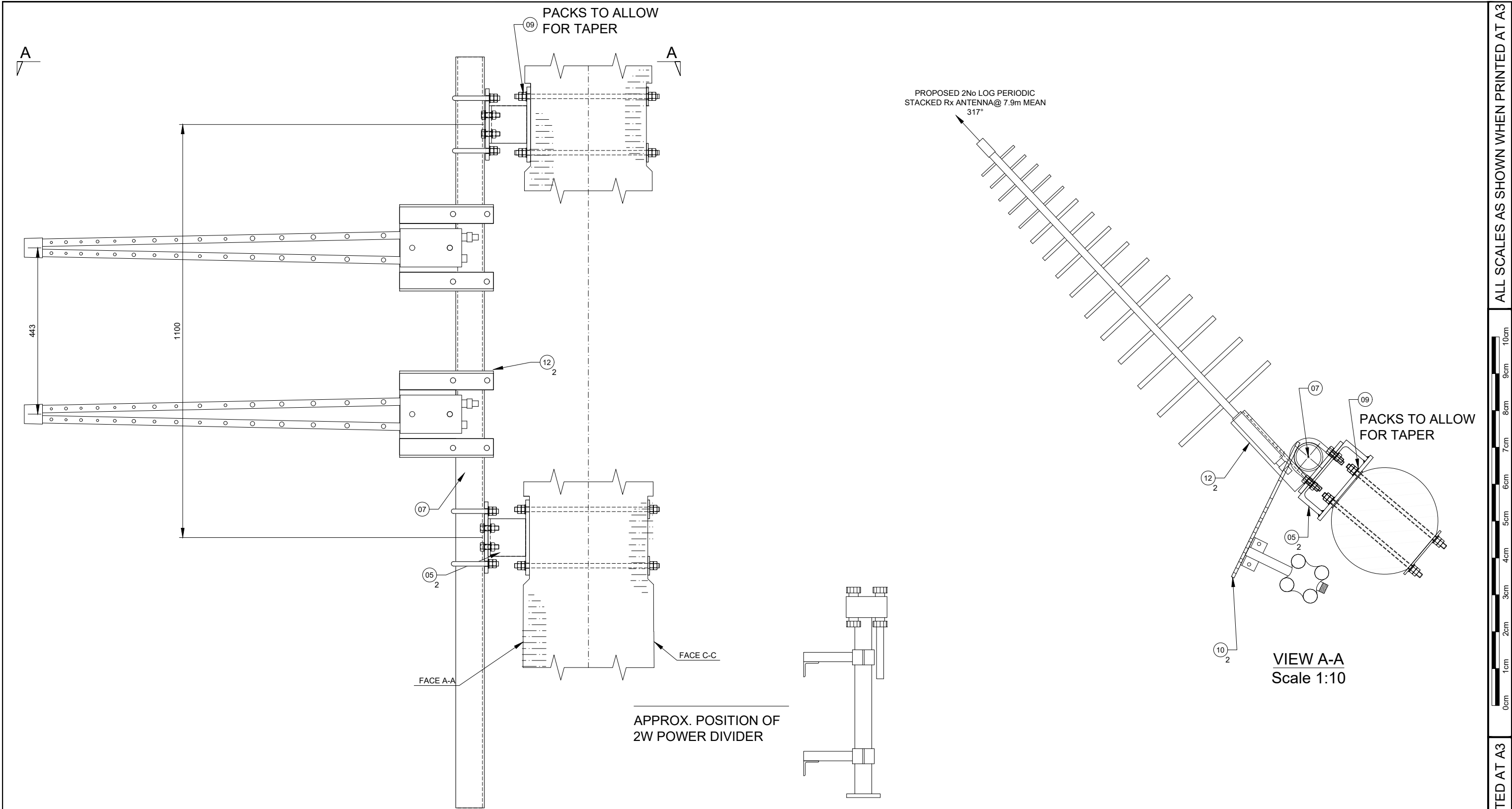
DETAIL I - Rx ANTENNA MOUNT Scale 1:10
