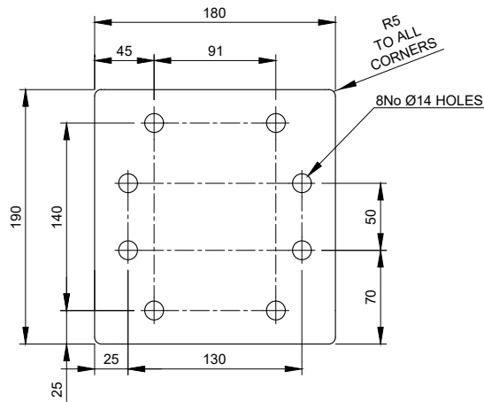
TPB-B-5 - 10mm THICK Scale 1:5
