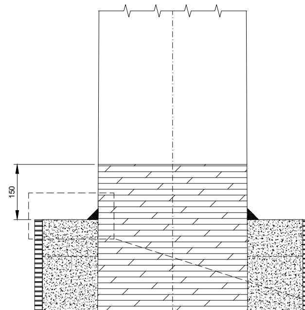
WATER PROOFING Scale 1:10
