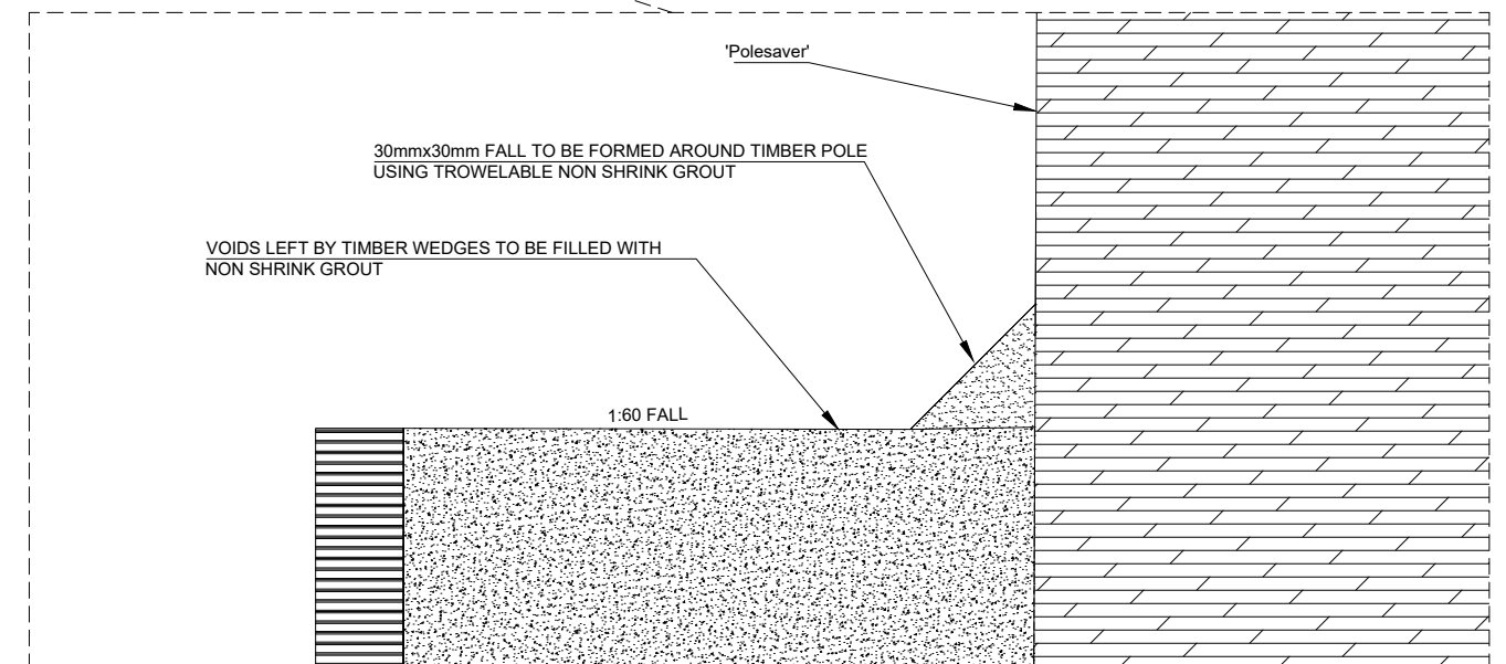
ENLARGED DETAIL Scale 1:2
