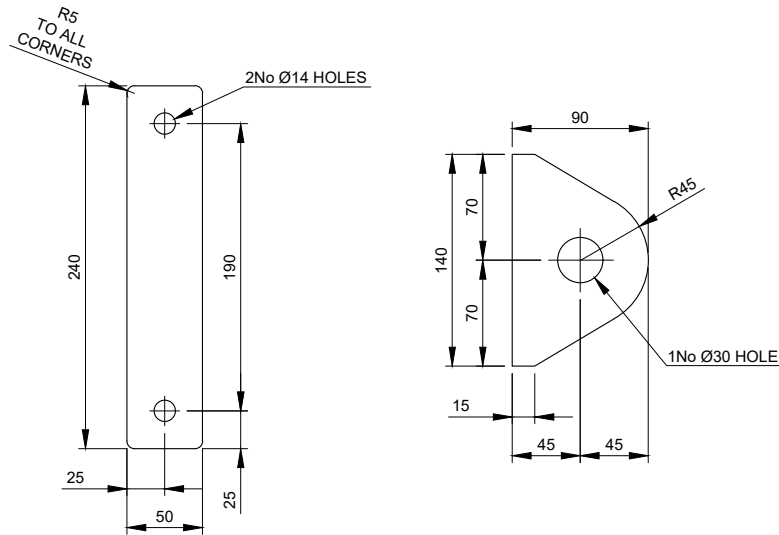
TPB-C-1 - 10mm THICK Scale 1:5 TPB-C-2 - 10mm THICK Scale 1:5
