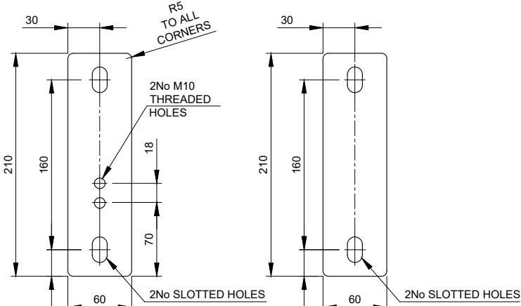
PART TPS-R-1 Scale 1:5 PART TPS-R-2 Scale 1:5
